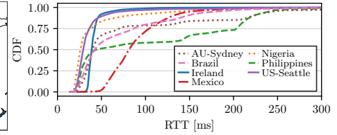
Figure 6: Starlink latency distribution from select cities in each continent.
